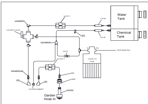
Plumbing Diagram
