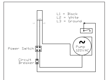
Wiring Diagram
